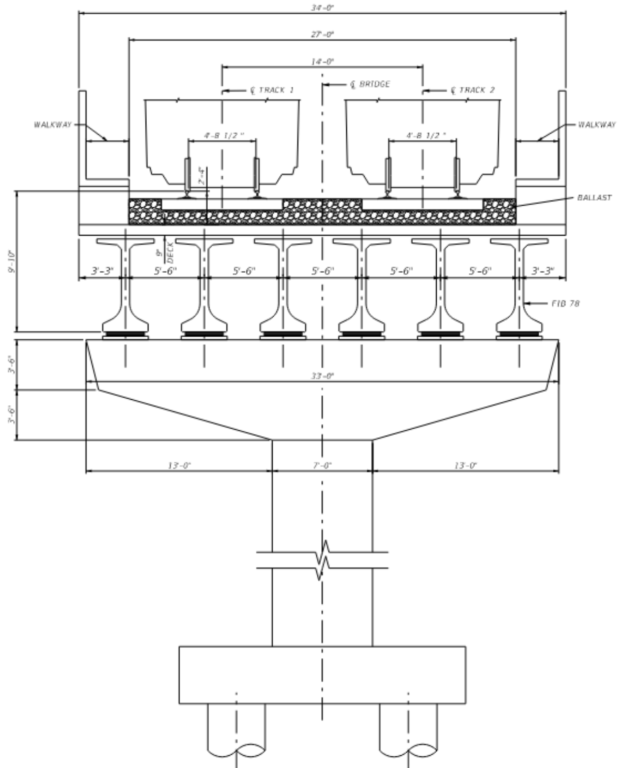
Figure 3-3: Guideway North & South Approaches FIB 78 – 119'-3" FT Spans
